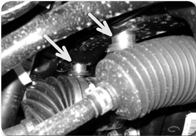
Figure 5 - Passenger Side with spacers installed
