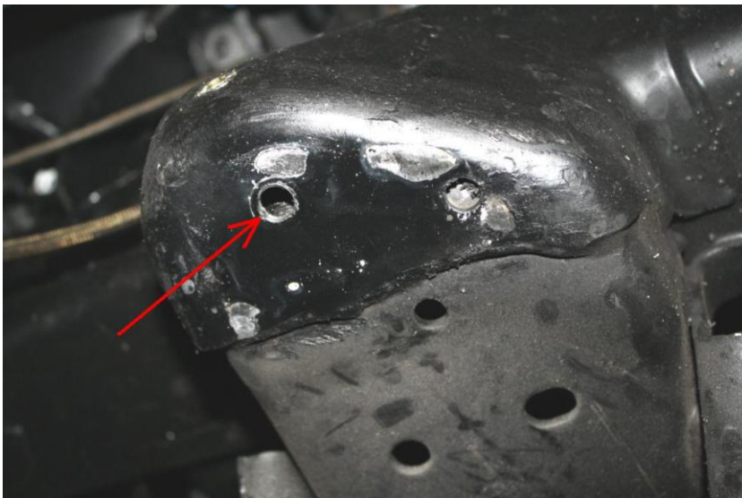
Figure 10: Rivet Nut Installation Location
