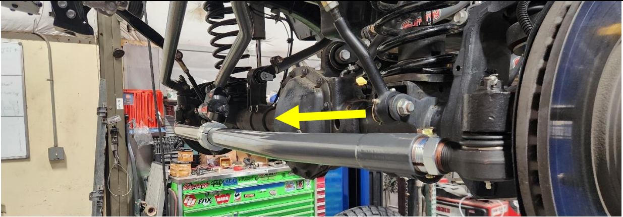
Figure 4. Synergy MFG Tie Rod With Bends Pointing Forward
