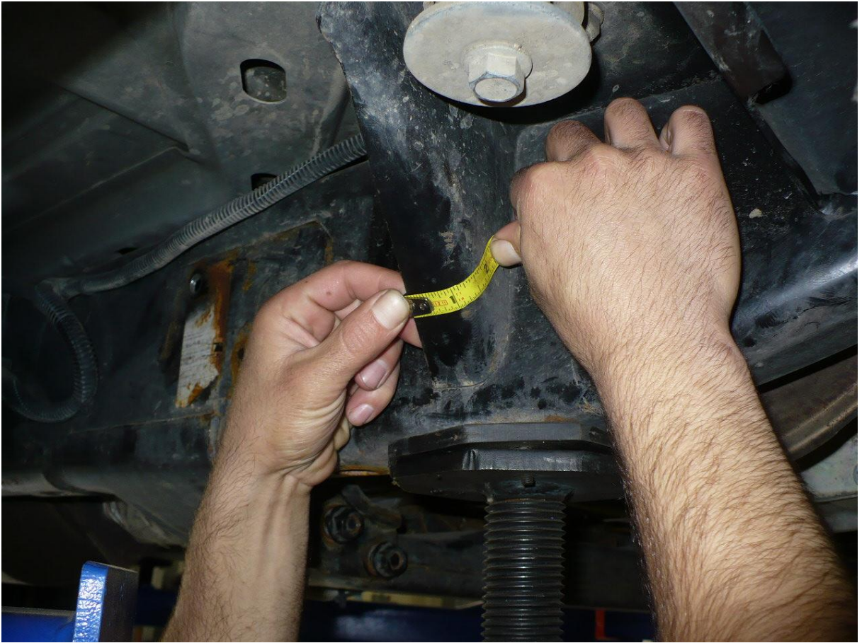
11) Trimmed drivers side body mount should appear as shown below.
