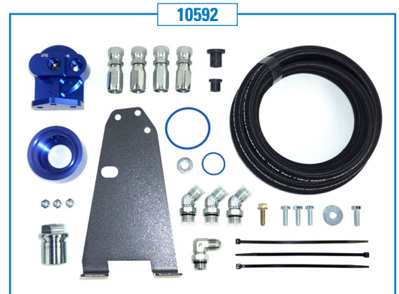
2003 - 2009 DODGE RAM 2500/3500 5.9L & 6.7L CUMMINS OIL FILTER THREAD OF 1 - 16 UN
