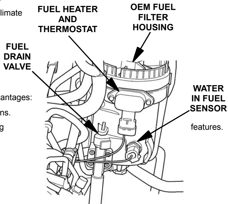
OEM FUEL FILTER HOUSING FEATURES
