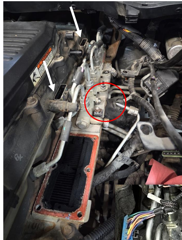
Figure 14: Injector harness disconnected, high pressure feed line circled.
