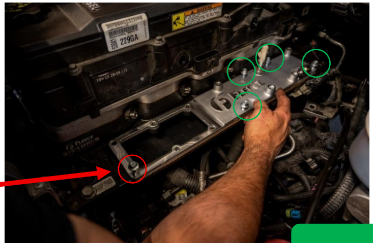
Figure 21: Intake plenum installed, M8 1.25x25 bolts circled.
