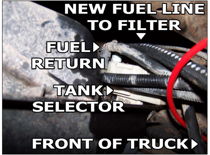
FIGURES 5 & 6 – SELECTOR VALVE VIEWS
