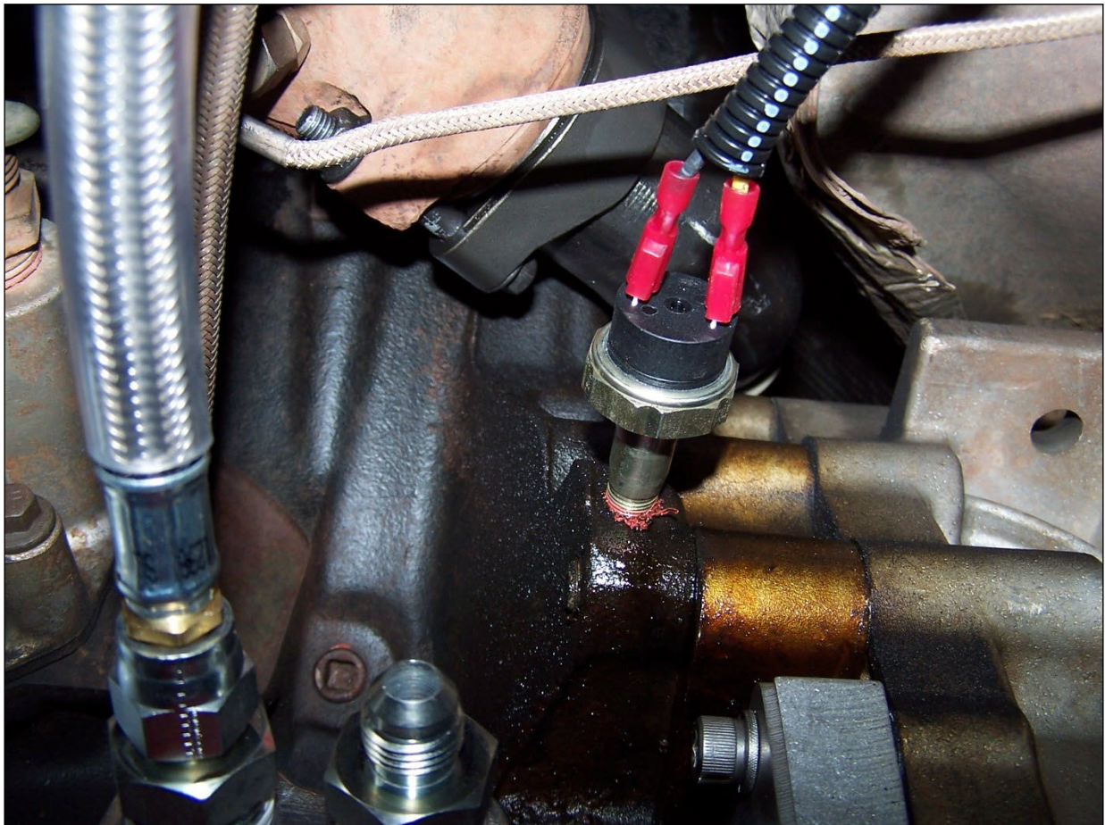
FIGURE 7 – OIL PRESSURE SWITCH INSTALLED – DRIVERS SIDE OF ENGINE BEHIND OIL FILTER
