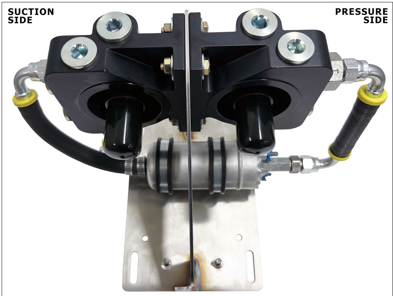
FIGURE 2 – FRONT VIEW OF ASSEMBLED FILTER/PUMP BRACKET (INSIDE FRAME ORIENTATION)
