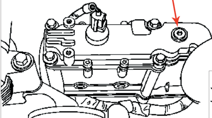
High Pressure Oil Pump Reservoir Plug
