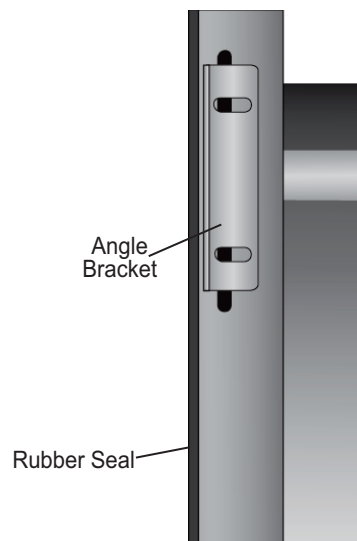
Option 2 Recessed Mount
