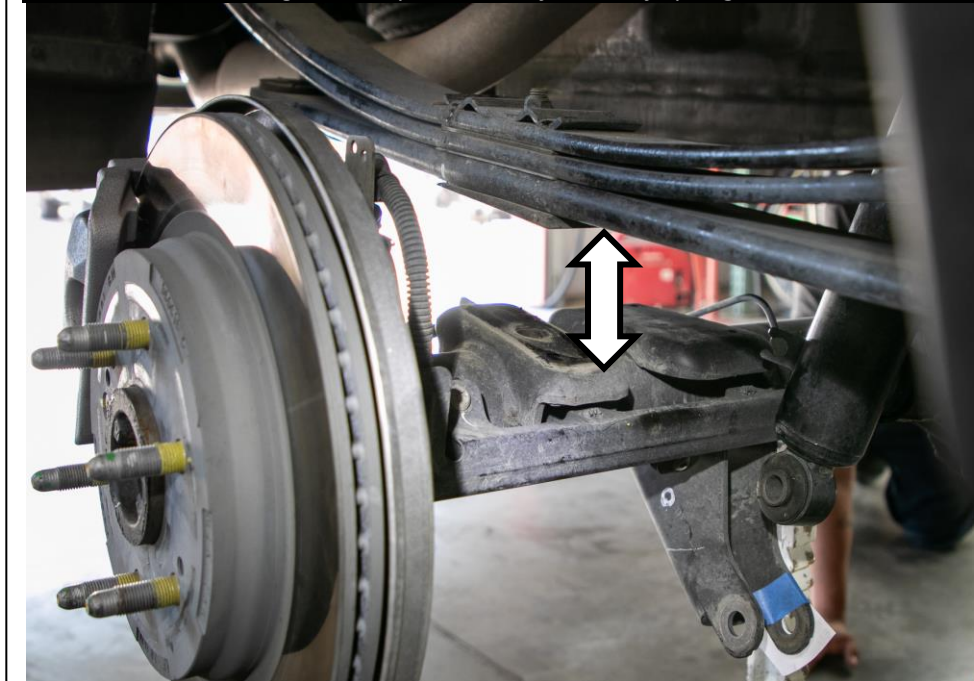
Figure 3: Separate Axle from Leaf Spring.
