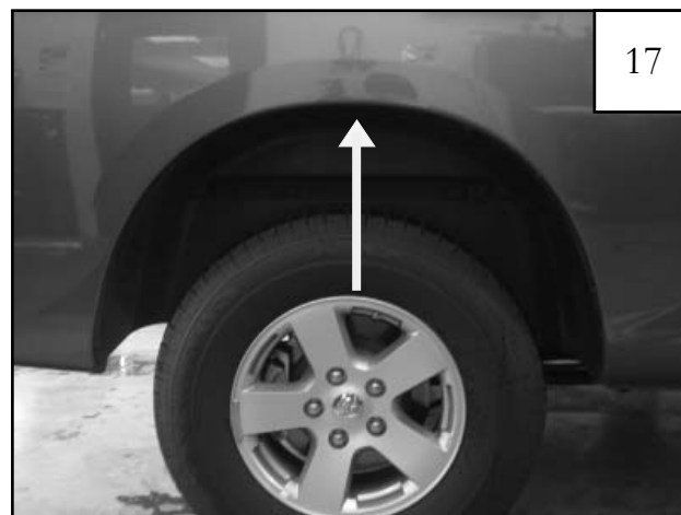
Install Clip (CL1-0022) in this location. See Steps 18, 19 & 20.
