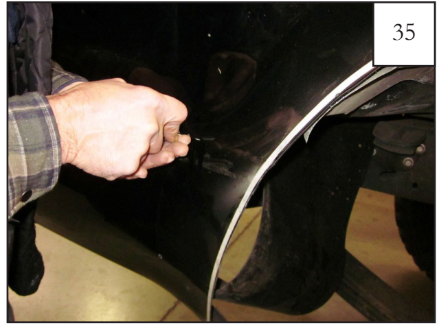
35 Remove flare. Using marks made with scratch awl as a guide, score the sheet metal with a center punch prior to drilling.
