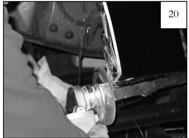
Using a hammer and an angle grinder, flatten tabs then grind down any sharp edges.
