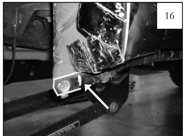
Using a grease pencil, make a line on flange at back of wheel well parallel to the outer edge. Using a cut-off wheel, cut away flange area indicated. DO NOT CUT BACK WALL OF WHEEL WELL. See step 17.
