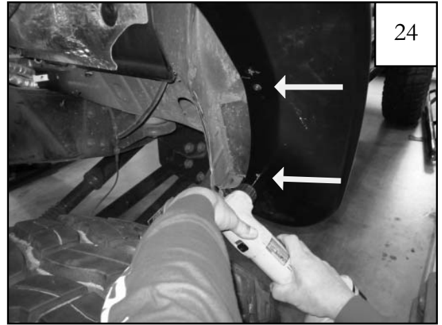
Hold flare tightly against fender, lining it up along style lines, drill into sheet metal through pre-drilled flare holes at rear side using 1/8" drill bit.
