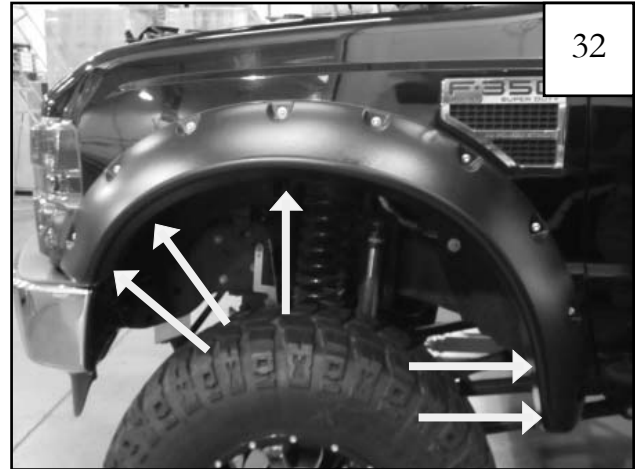
Install flare using screw (SW1-0056) through holes indicated.
