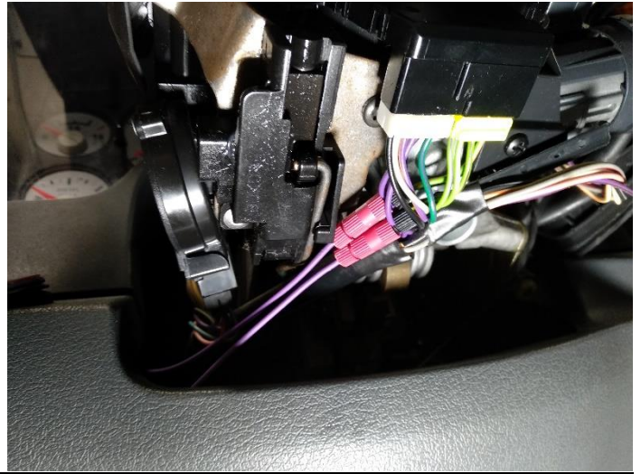
Clock spring C1 (WHITE) Pinout (2005-2007)
