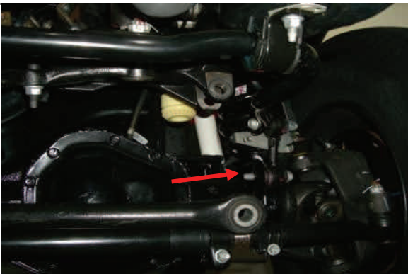
05-10 Disconnect lower sway bar mounting hardware
