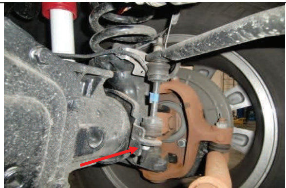
2011-UP Disconnect lower sway bar mounting hardware
