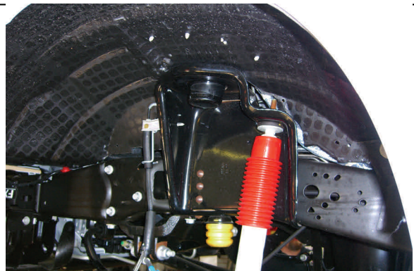
Carefully lower axle and remove coil spring
