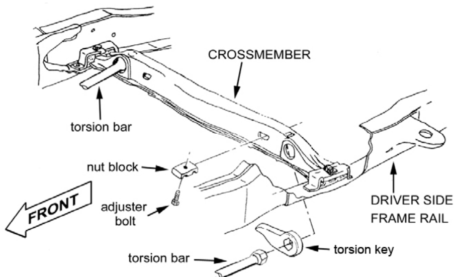
FIGURE 1 - TORSION BAR ASSEMBLY.
