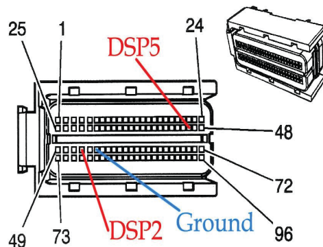
STEP 6 PIN-OUT REFERENCE (VIEWED LOOKING AT CONNECTOR FACE)
