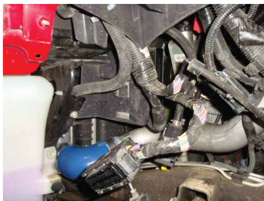
STEP 4 REMOVE TOP COVER
