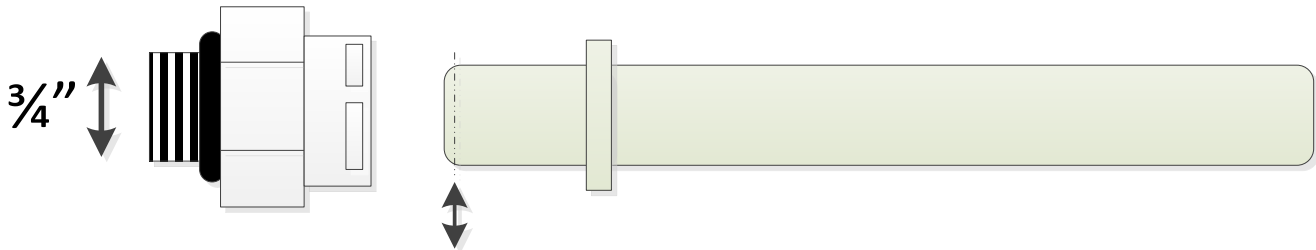
Trim a small 1/16" from the tip of the transmission cooler line. Leave no sharp edges.
