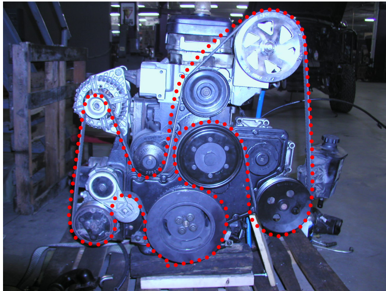
Figure 17: Belt Routing
