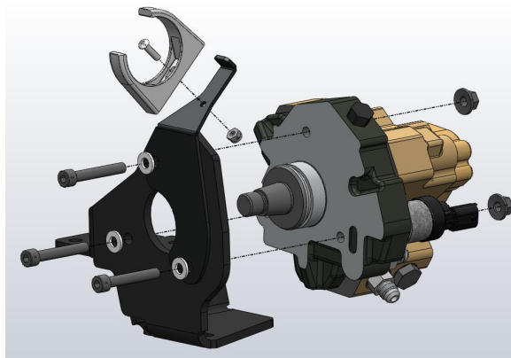
Figure 7 - Pump Bracket Assembly
