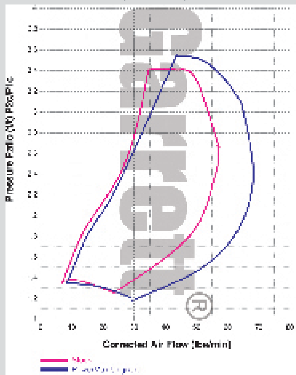
Compressor Map
