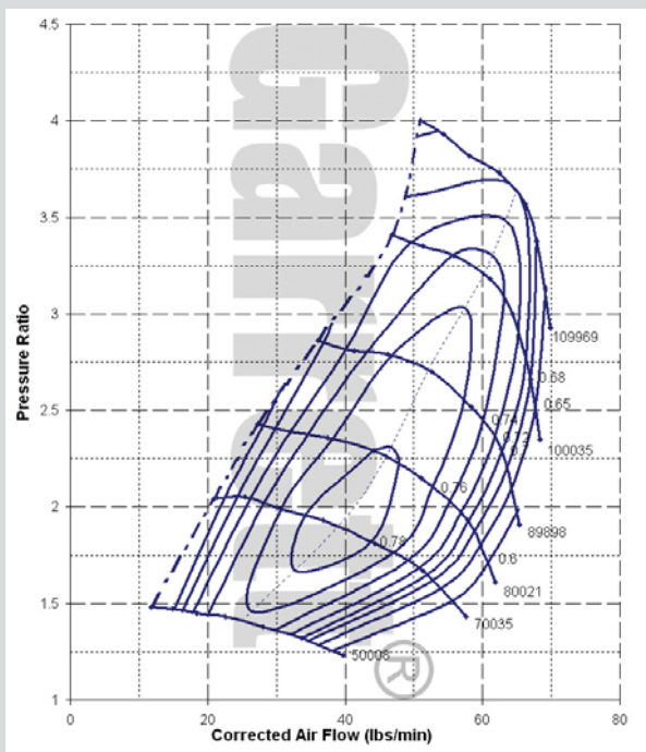
Compressor Map
