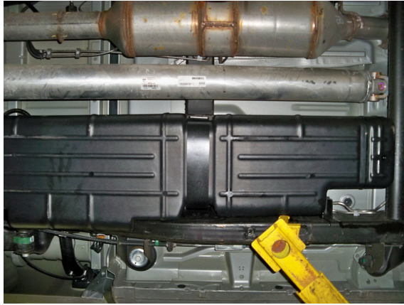
(Fig. 17) 7010211 Installation showing optional TITAN Shield.
