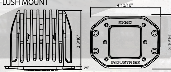
FLUSH MOUNT
